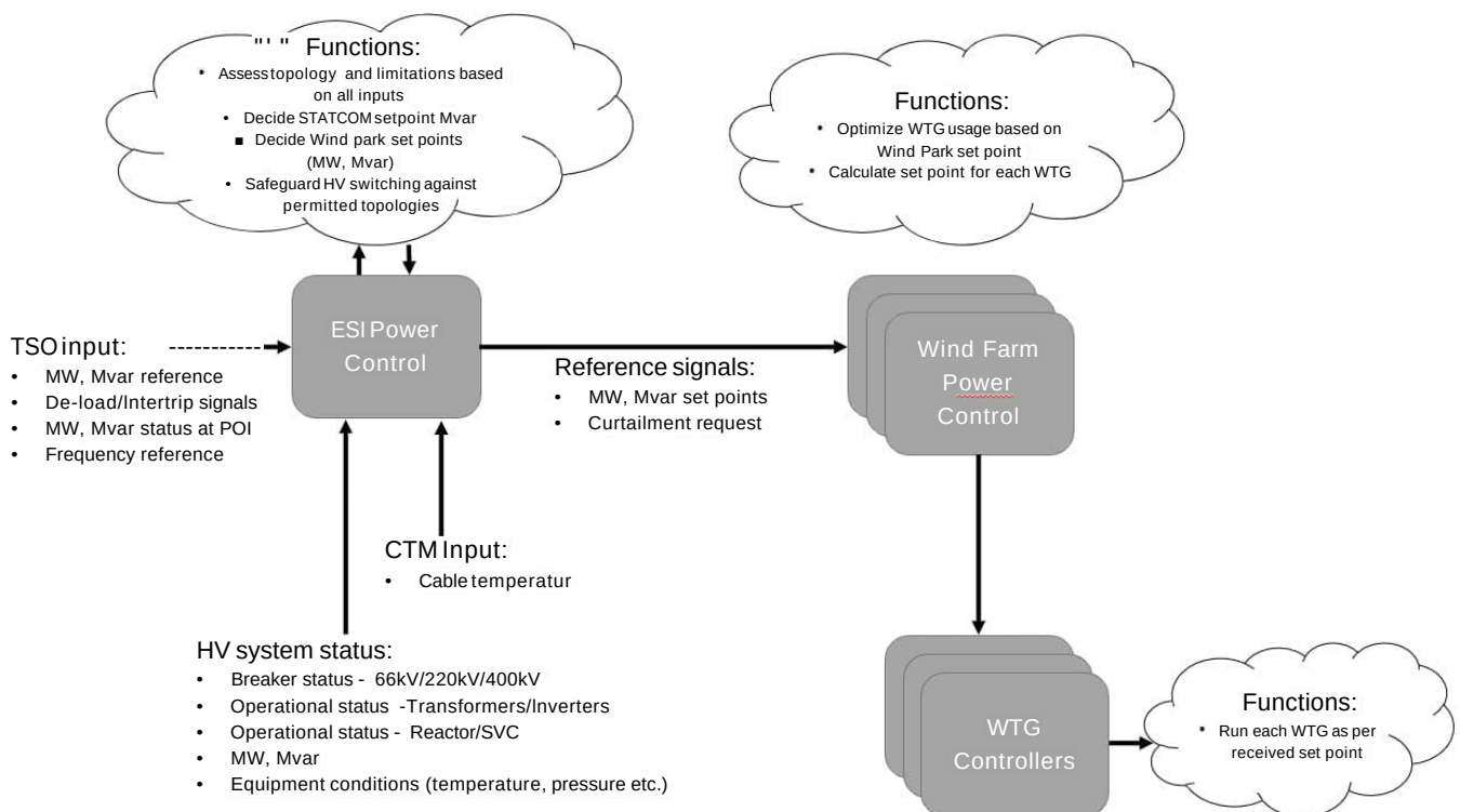
Figure 2 Power Control, Interlocks and Grid Compliance. ESI Power control to be delivered by ESI contractor. WFPC and WTG controllers are WTG delivery.
